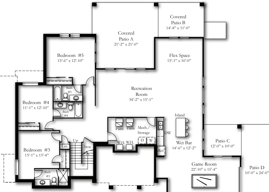
Basement Plan A Total 2,624 Sq. Ft. Finished 2,398 Sq. Ft.
